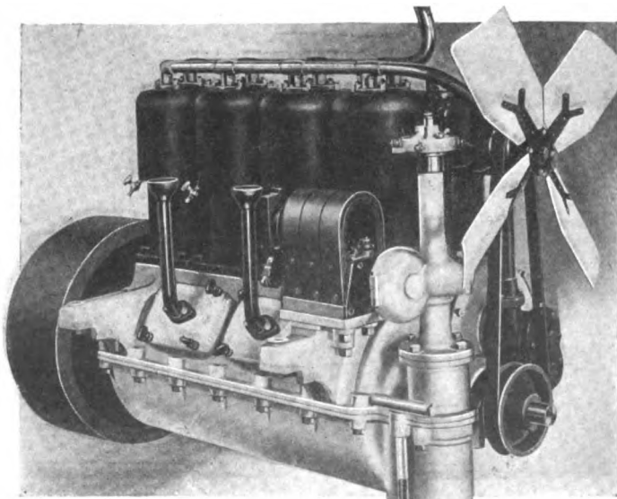
Individual Cylinder Motor with Magneto.
